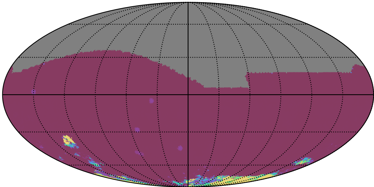
noroll_mjdp0_v3.4_10yrs All sky iz bands: 75th Percentile Intranight Timespan
