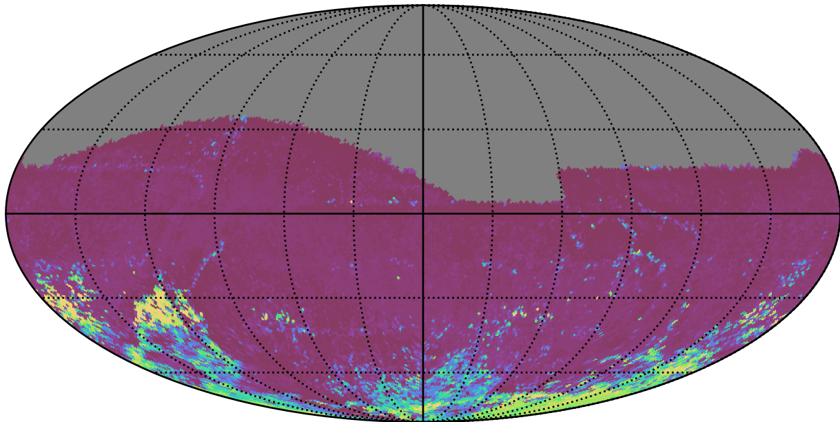
noroll_mjdp0_v3.4_10yrs All sky i band: 75th Percentile Intranight Timespan
