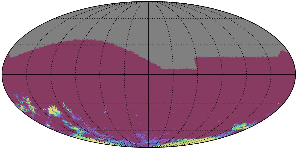
noroll_mjdp0_v3.4_10yrs All sky gr bands: 75th Percentile Intranight Timespan
