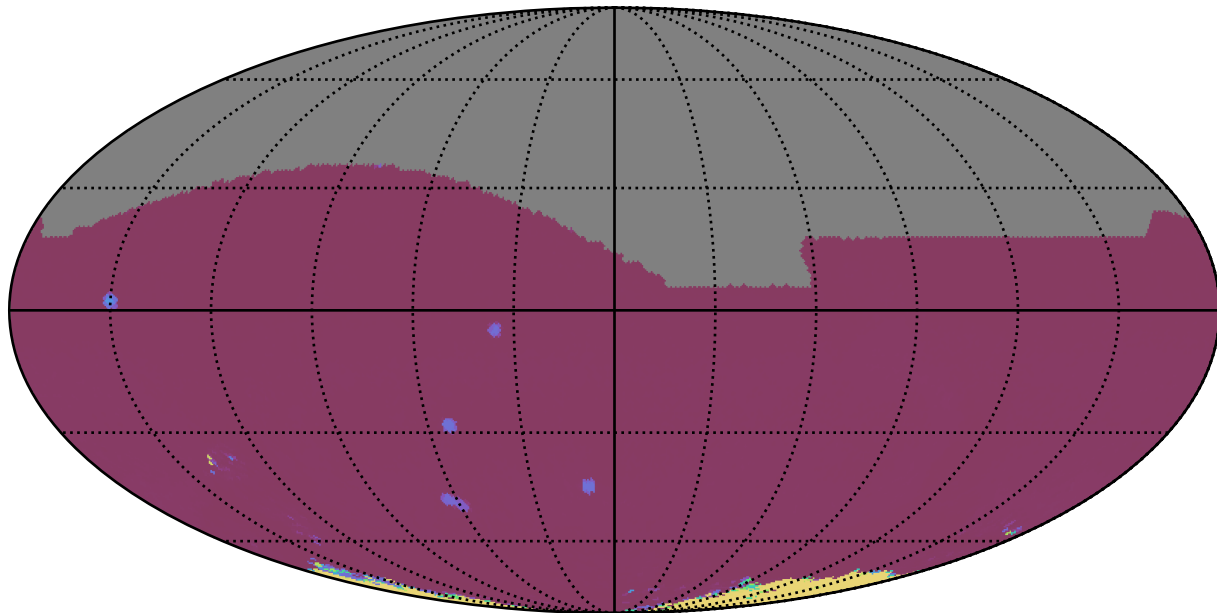
noroll_mjdp0_v3.4_10yrs All sky: 75th Percentile Intranight Timespan
