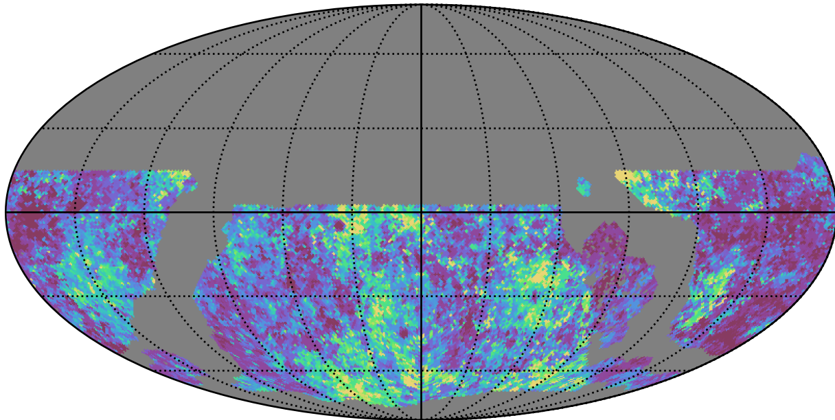
noroll_mjdp0_v3.4_10yrs WFD g band: 20thPercentile Inter-Night Gap
