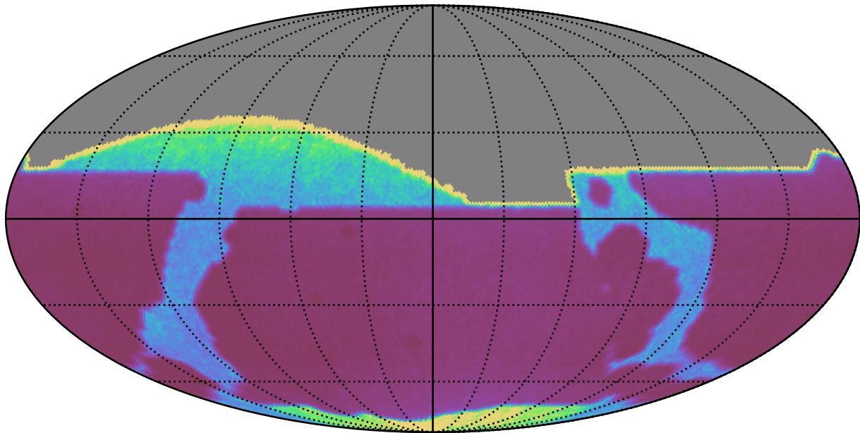
noroll_mjdp0_v3.4_10yrs : properMotion
