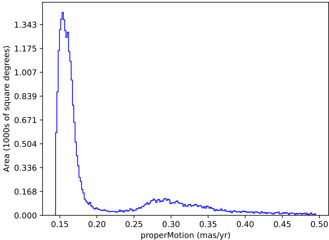
noroll_mjdp0_v3.4_10yrs : properMotion
