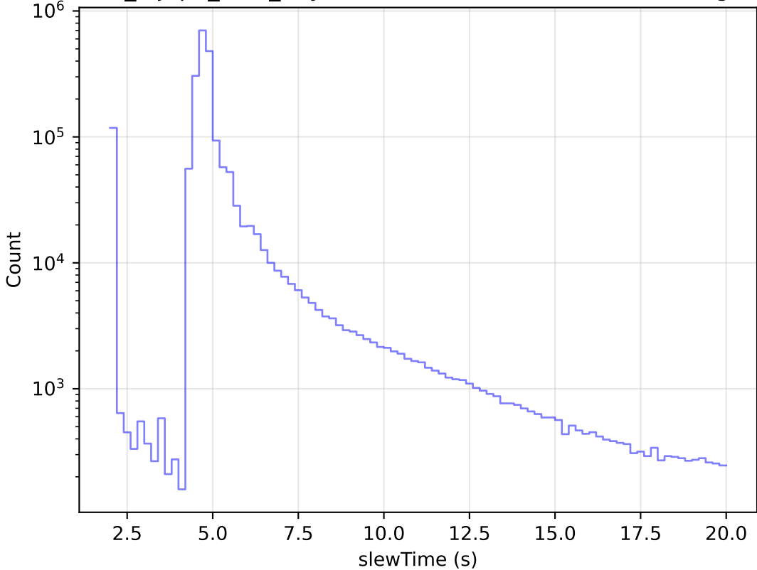
noroll_mjdp0_v3.4_10yrs All visits: Zoom Slew Time Histogram
