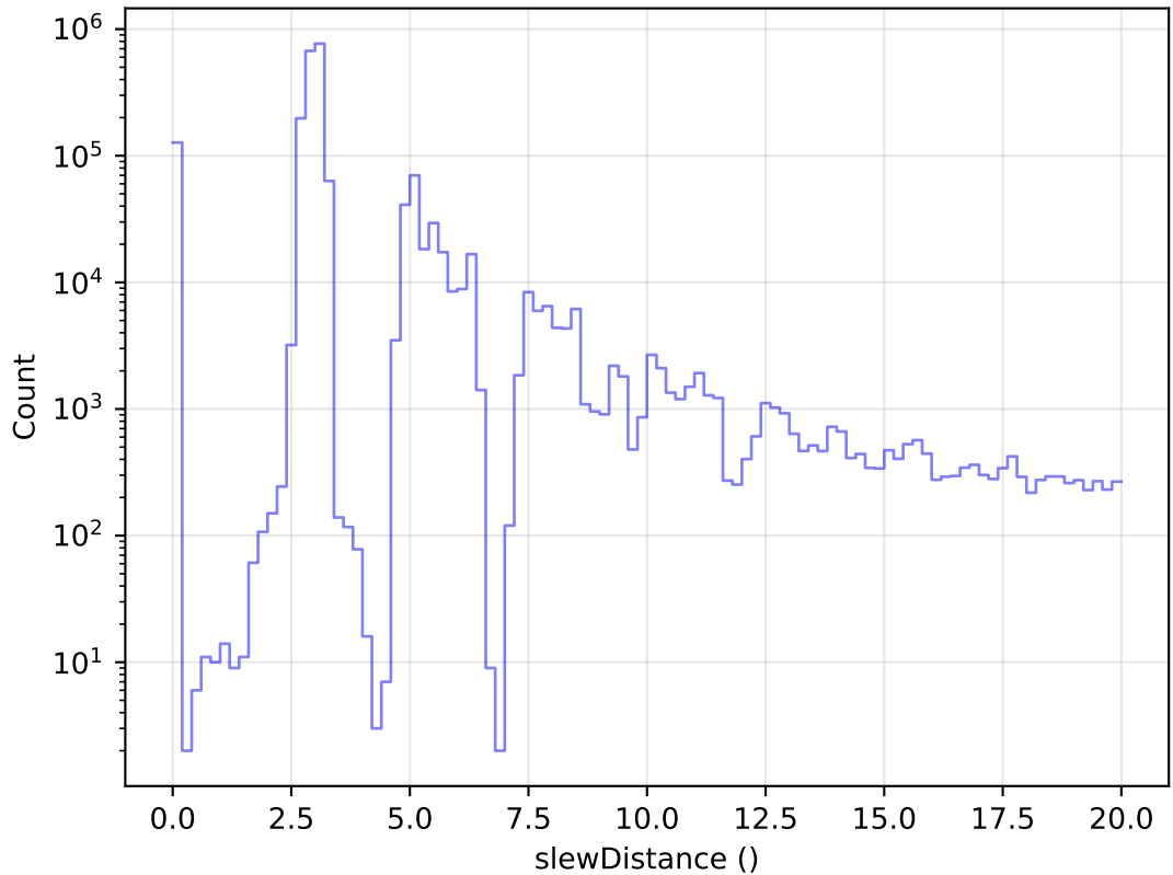
noroll_mjdp0_v3.4_10yrs All visits: Zoom Slew Distance Histogram
