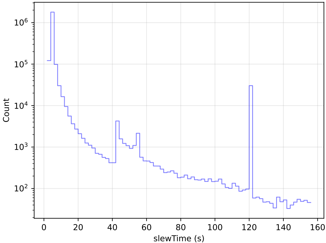
noroll_mjdp0_v3.4_10yrs All visits: Slew Time Histogram
