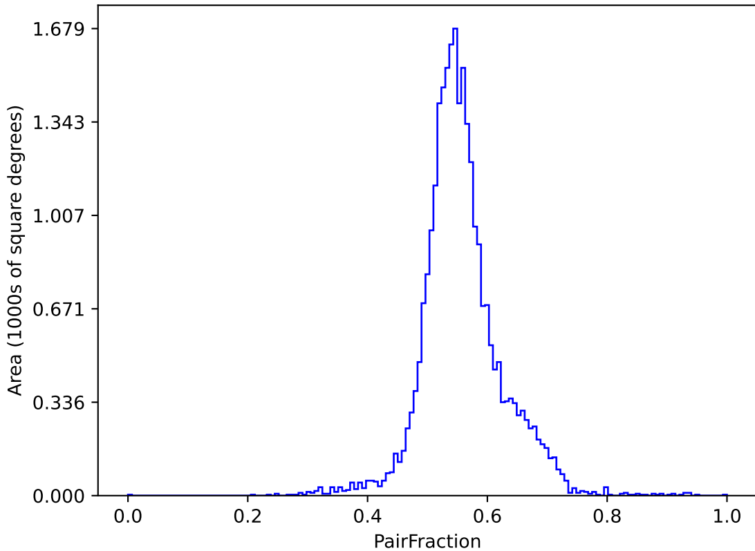
noroll_mjdp0_v3.4_10yrs (g or r or i): PairFraction
