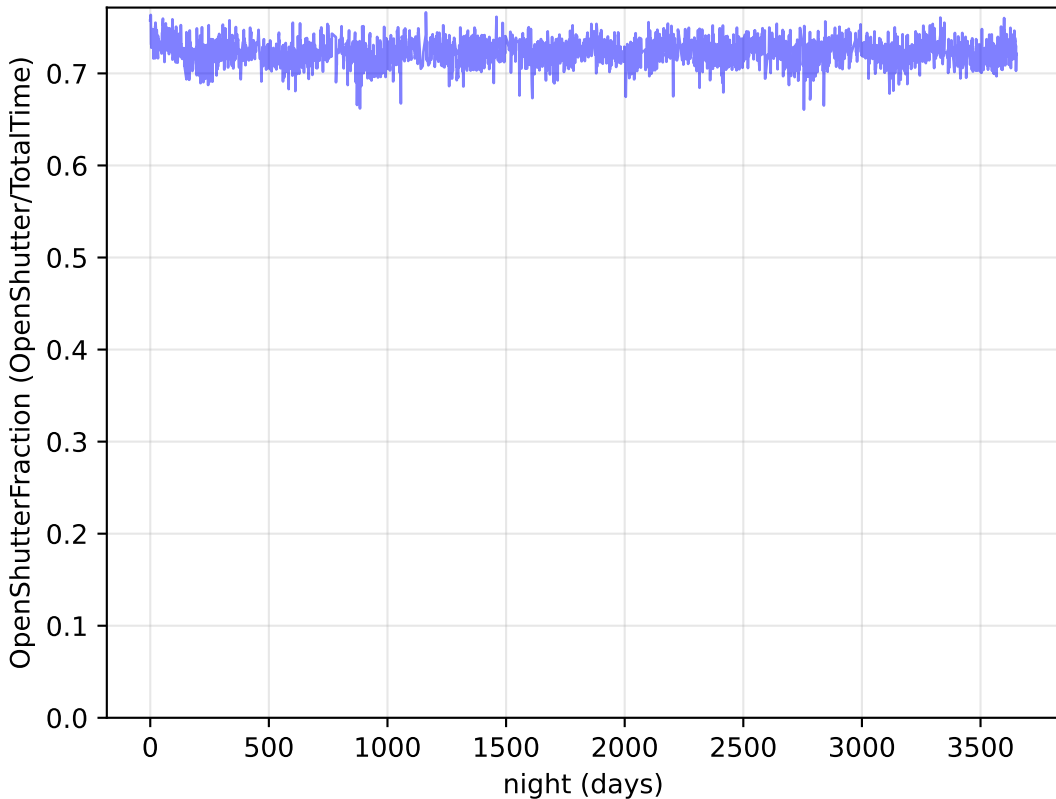
noroll_mjdp0_v3.4_10yrs : OpenShutterFraction
