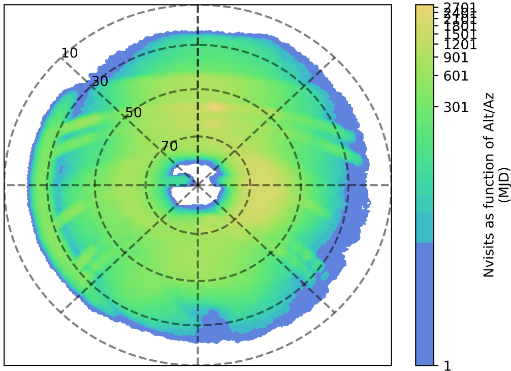
noroll_mjdp0_v3.4_10yrs r: Nvisits as function of Alt/Az
