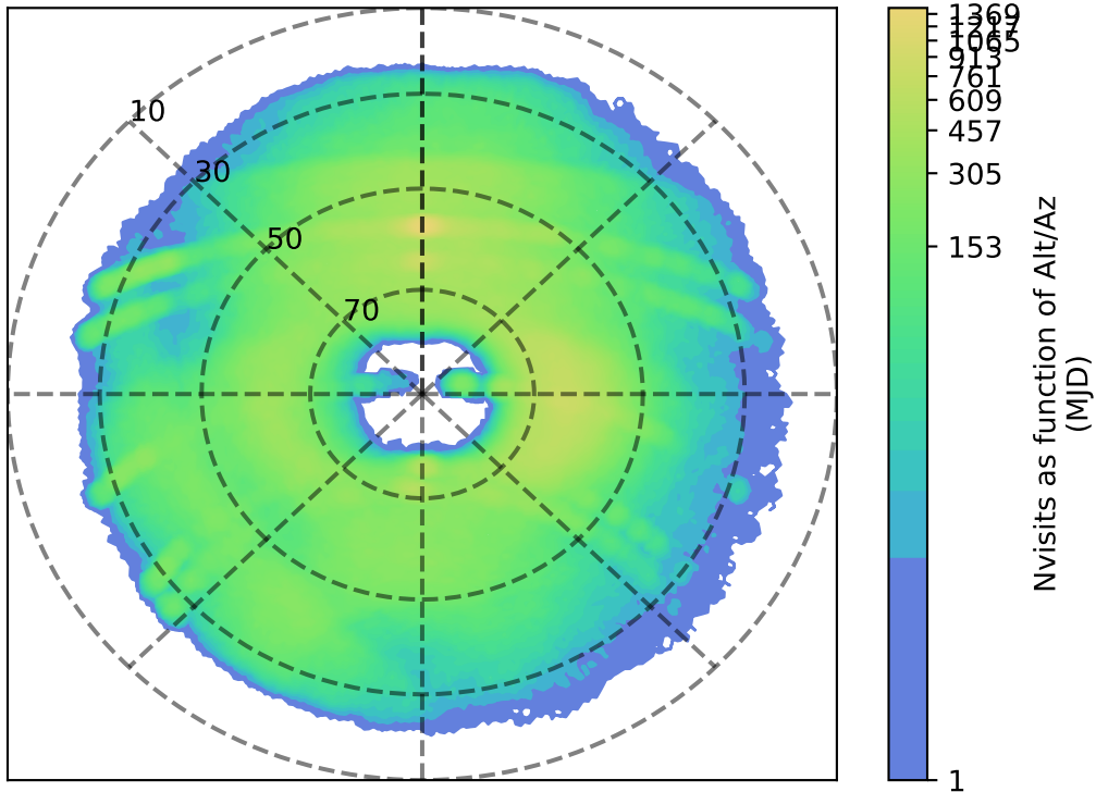
noroll_mjdp0_v3.4_10yrs g: Nvisits as function of Alt/Az
