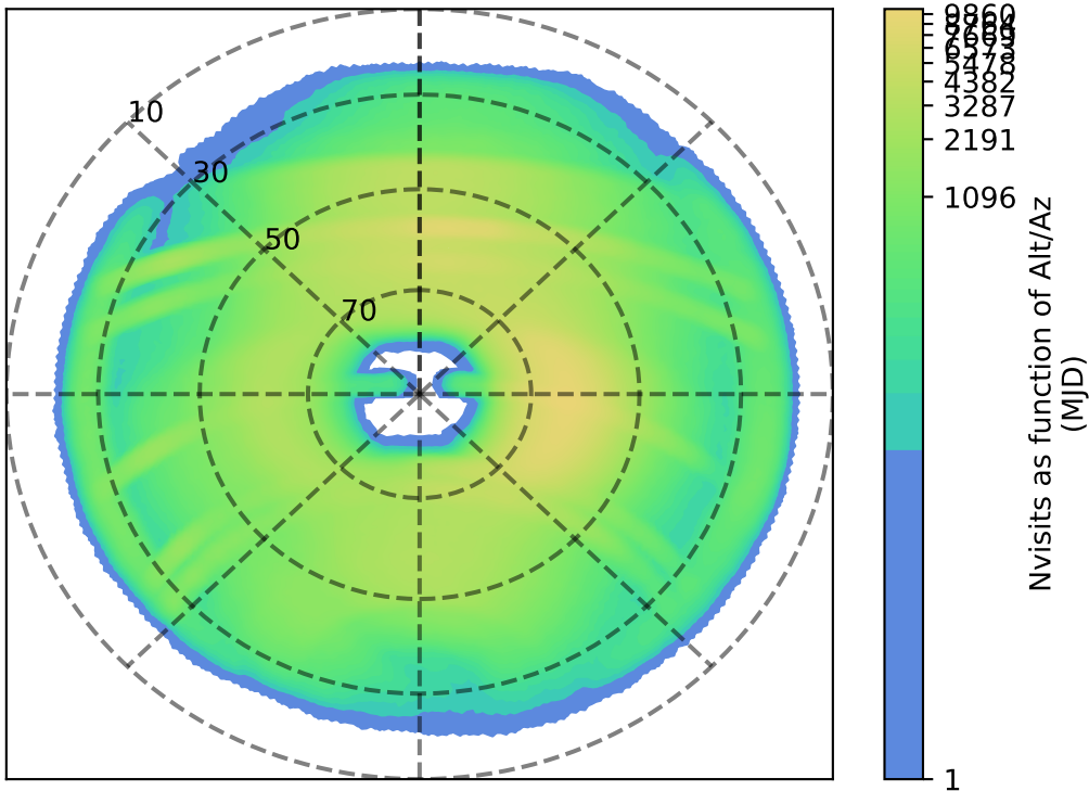
noroll_mjdp0_v3.4_10yrs : Nvisits as function of Alt/Az
