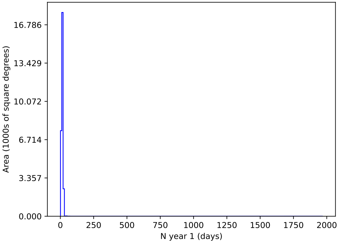
noroll_mjdp0_v3.4_10yrs z and night < 365: N year 1
