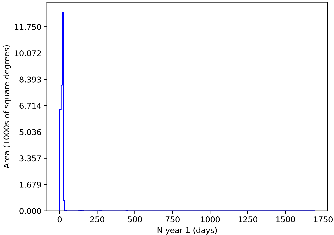
noroll_mjdp0_v3.4_10yrs r and night < 365: N year 1
