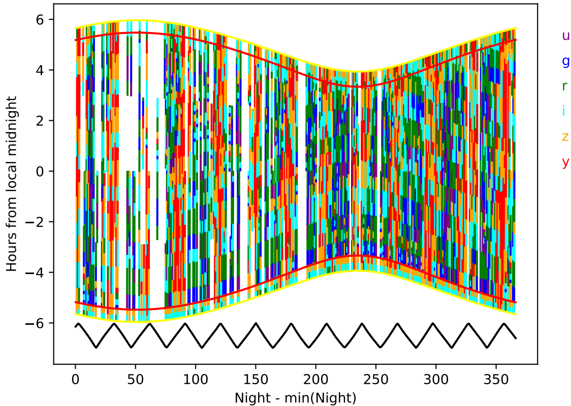
noroll_mjdp0_v3.4_10yrs year 9-10: Hourglass
