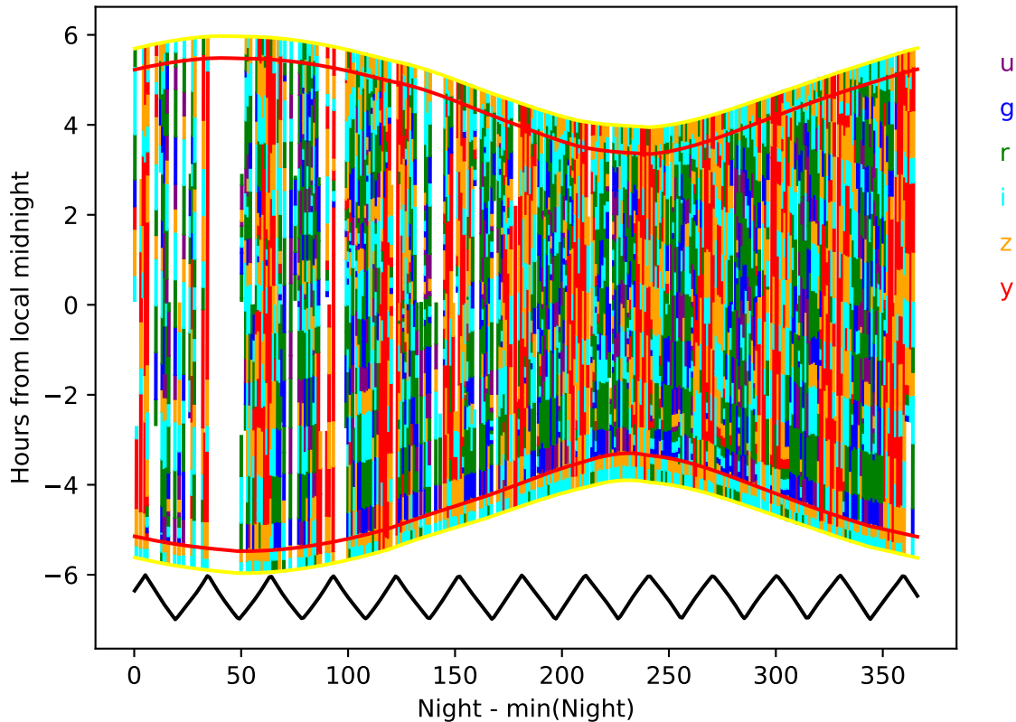
noroll_mjdp0_v3.4_10yrs year 6-7: Hourglass
