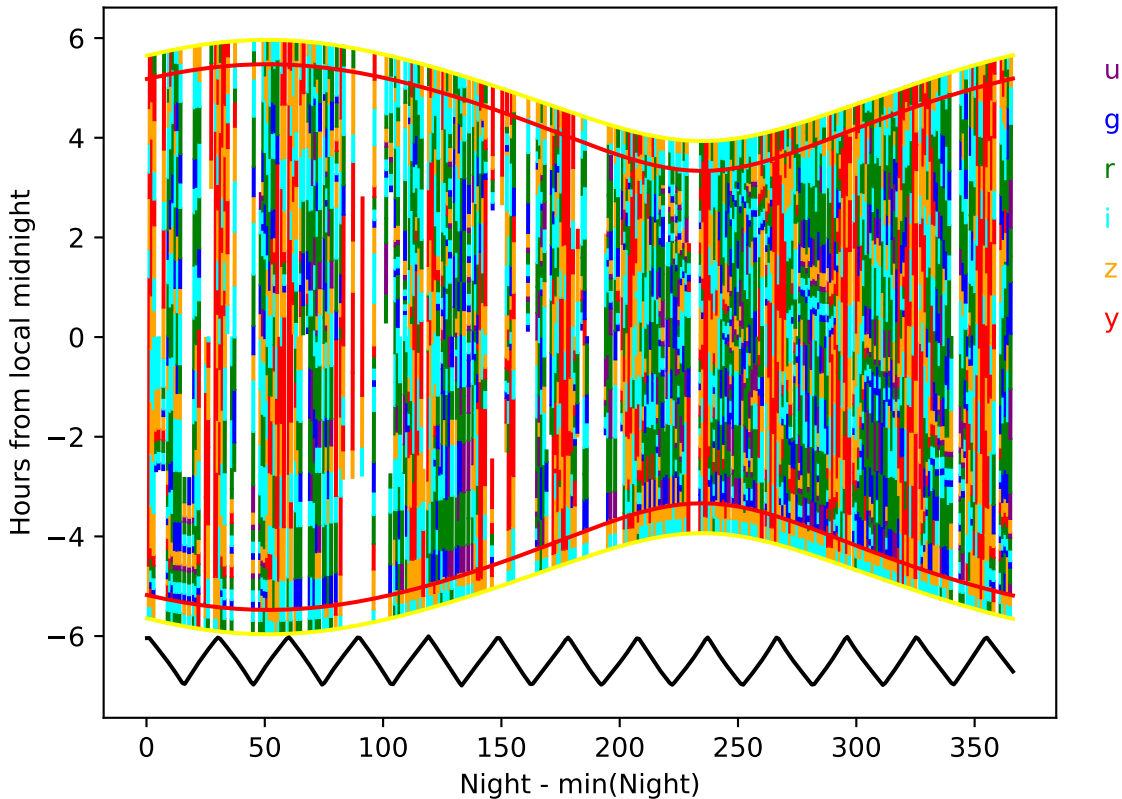
noroll_mjdp0_v3.4_10yrs year 1-2: Hourglass
