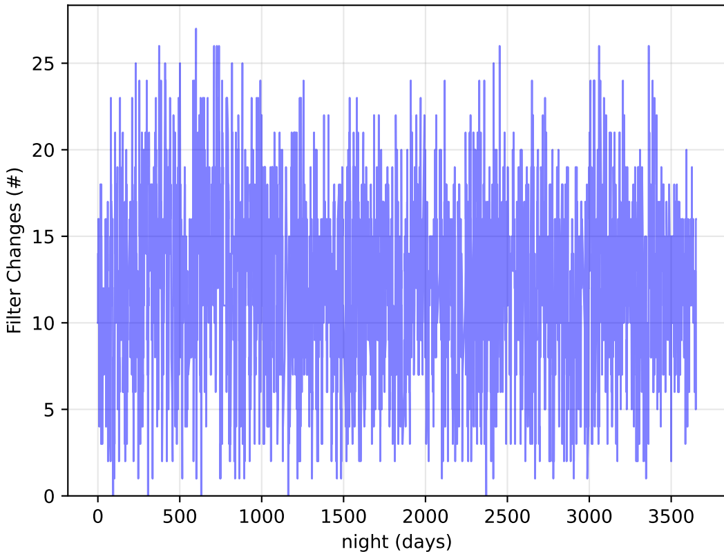
noroll_mjdp0_v3.4_10yrs : Filter Changes
