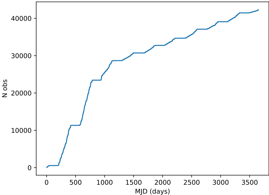
noroll_mjdp0_v3.4_10yrs note like DD:COSMOS%: Cumulative
