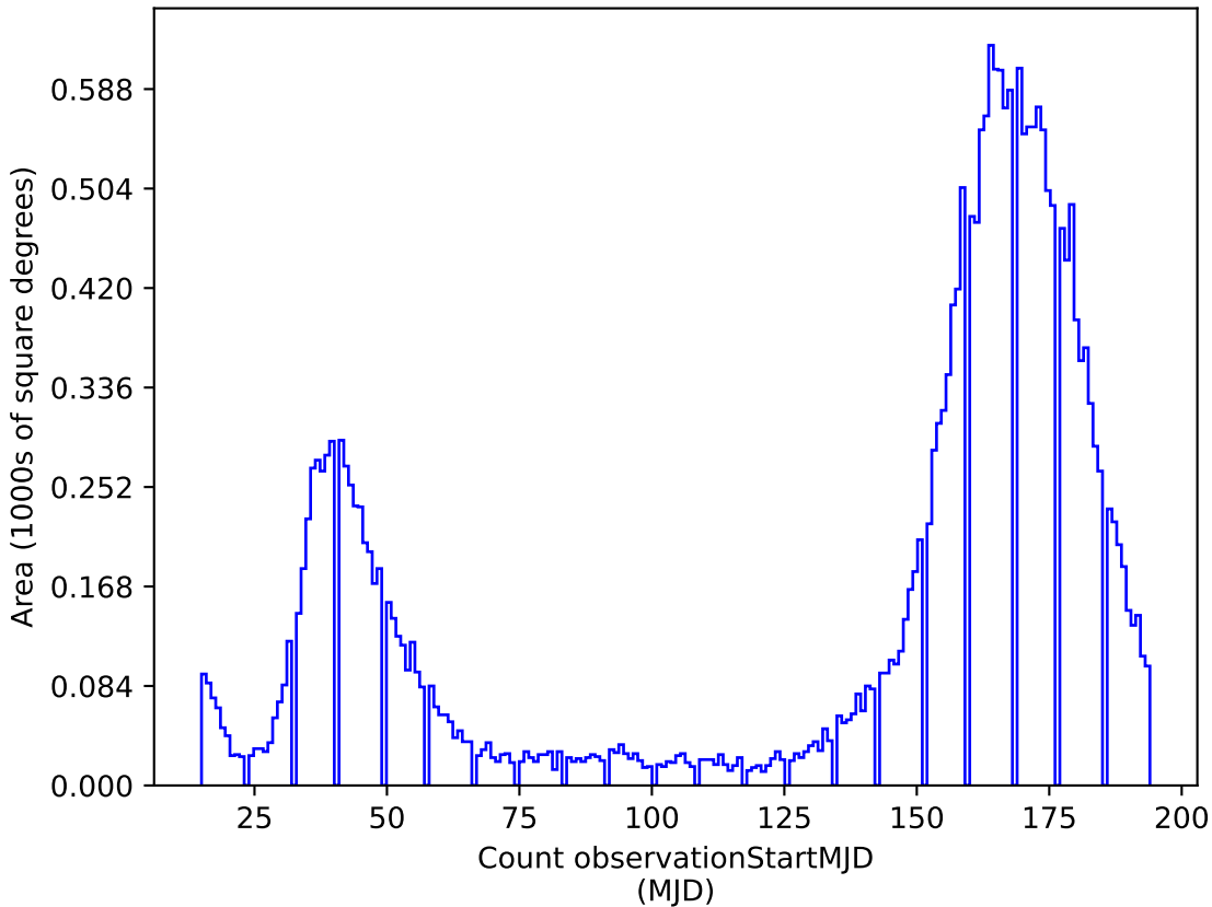
noroll_mjdp0_v3.4_10yrs z: Count observationStartMJD
