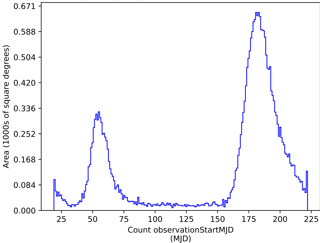
noroll_mjdp0_v3.4_10yrs r: Count observationStartMJD
