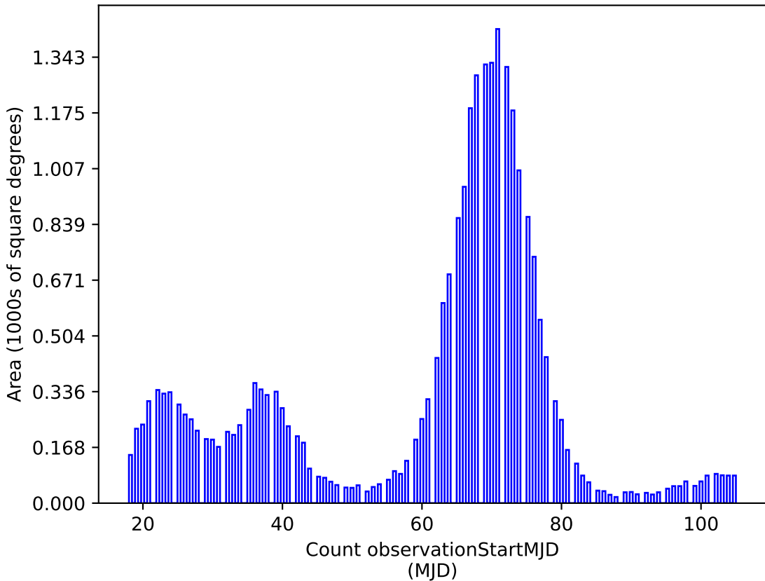
noroll_mjdp0_v3.4_10yrs g: Count observationStartMJD
