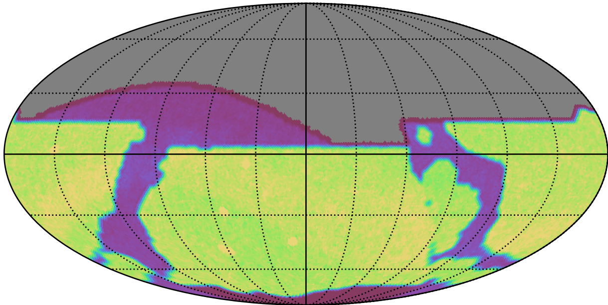
noroll_mjdp0_v3.4_10yrs : Count observationStartMJD
