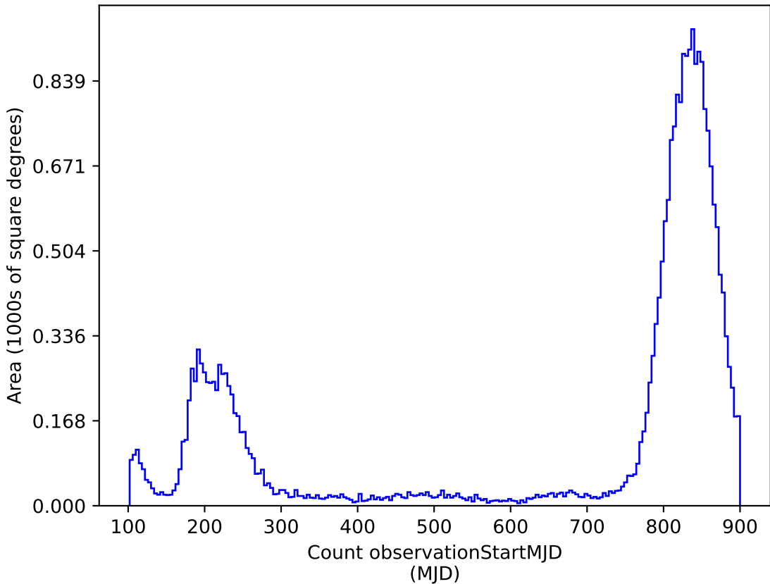
noroll_mjdp0_v3.4_10yrs : Count observationStartMJD
