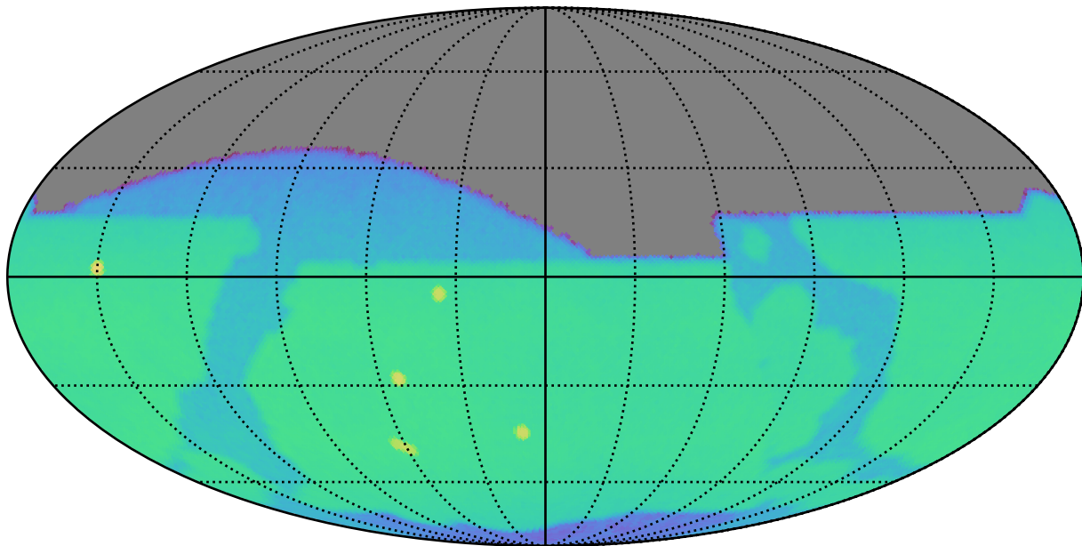
noroll_mjdp0_v3.4_10yrs z: CoaddM5
