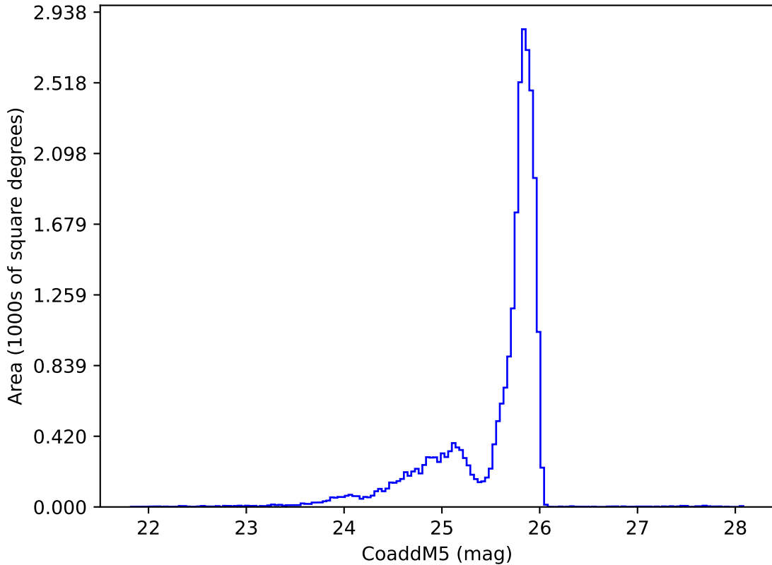
noroll_mjdp0_v3.4_10yrs z: CoaddM5
