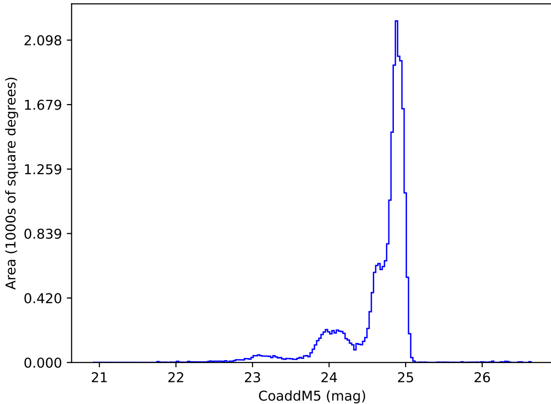
noroll_mjdp0_v3.4_10yrs y: CoaddM5
