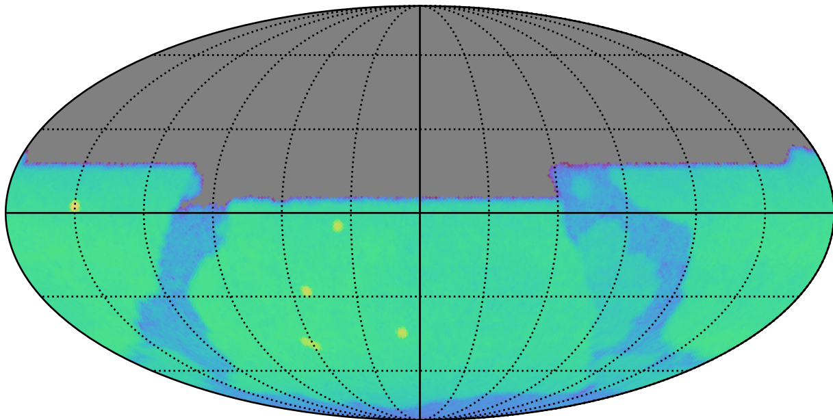
noroll_mjdp0_v3.4_10yrs u: CoaddM5
