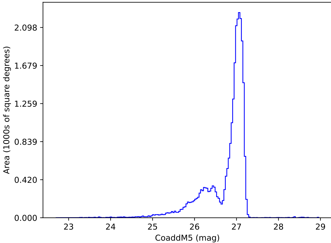
noroll_mjdp0_v3.4_10yrs r: CoaddM5
