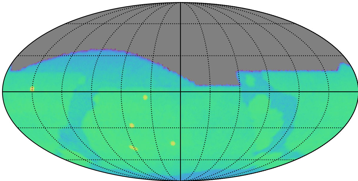
noroll_mjdp0_v3.4_10yrs g: CoaddM5
