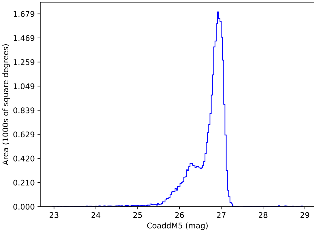
noroll_mjdp0_v3.4_10yrs g: CoaddM5
