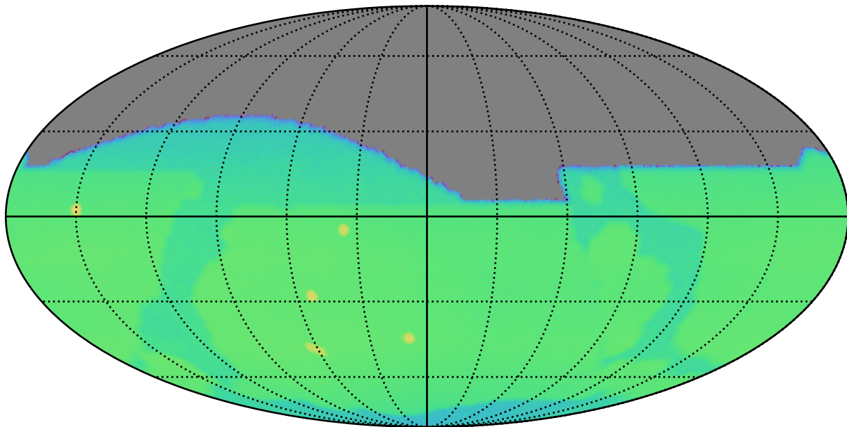
noroll_mjdp0_v3.4_10yrs : CoaddM5
