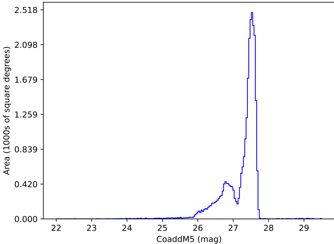
noroll_mjdp0_v3.4_10yrs : CoaddM5
