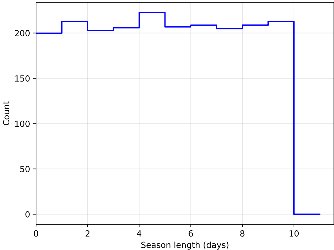
noroll_mjdp0_v3.4_10yrs DD:XMM_LSS all bands: SeasonLength
