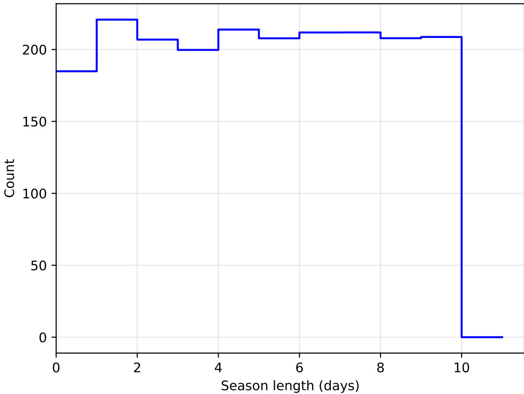
noroll_mjdp0_v3.4_10yrs DD:ELAISS1 all bands: SeasonLength
