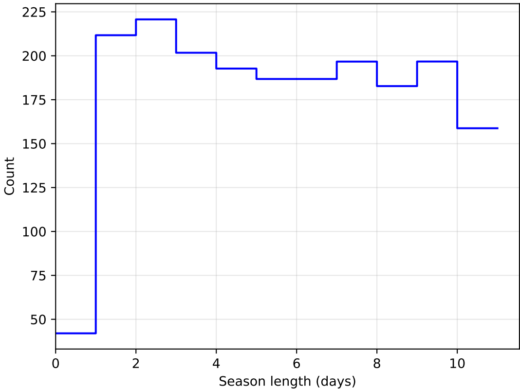
noroll_mjdp0_v3.4_10yrs DD: COSMOS all bands: SeasonLength
