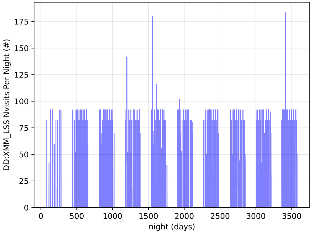
noroll_mjdp0_v3.4_10yrs all bands: DD:XMM_LSS Nvisits Per Night
