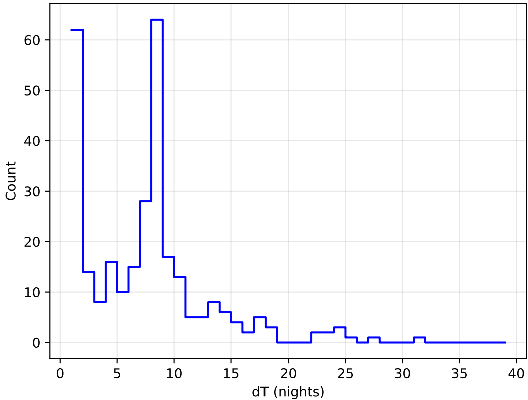
noroll_mjdp0_v3.4_10yrs all bands: DD:XMM_LSS Delta Nights Histogram
