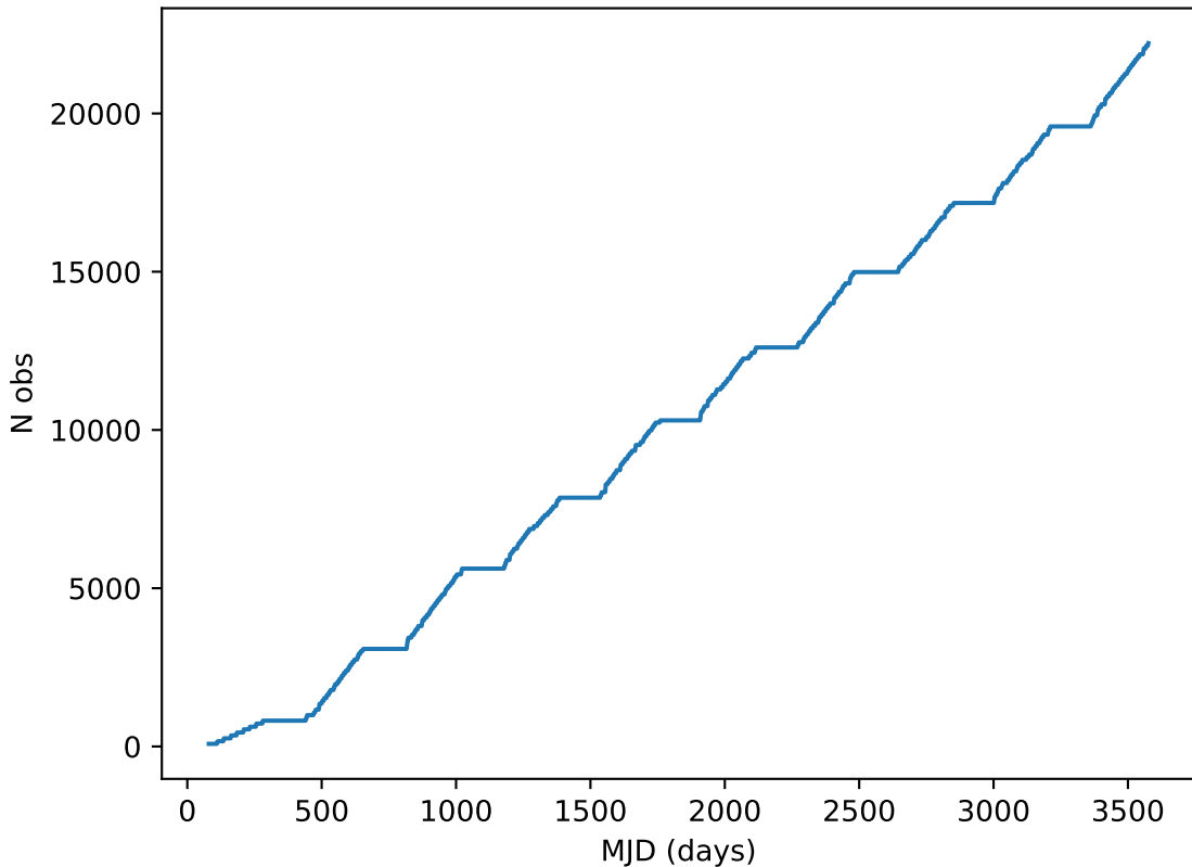
noroll_mjdp0_v3.4_10yrs all bands: DD:XMM_LSS Cumulative NVisits
