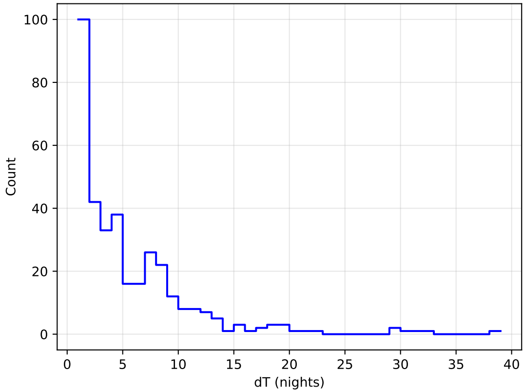
noroll_mjdp0_v3.4_10yrs all bands: DD:WFD Delta Nights Histogram
