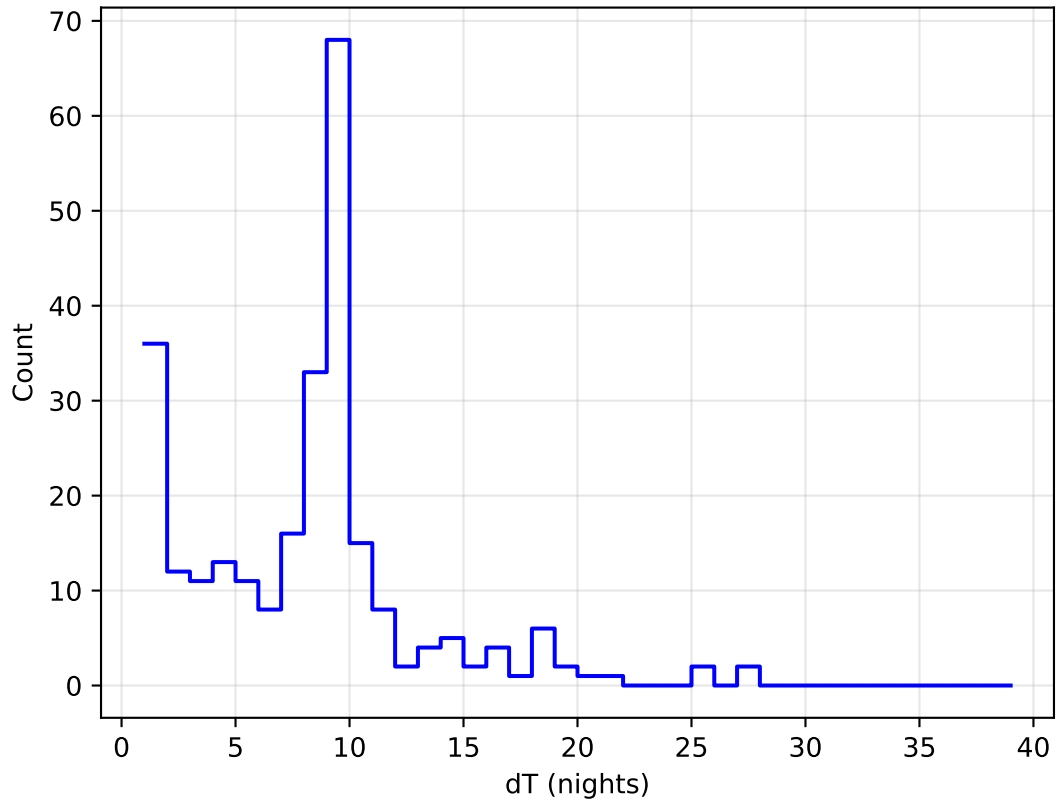
noroll_mjdp0_v3.4_10yrs all bands: DD:ELAISS1 Delta Nights Histogram
