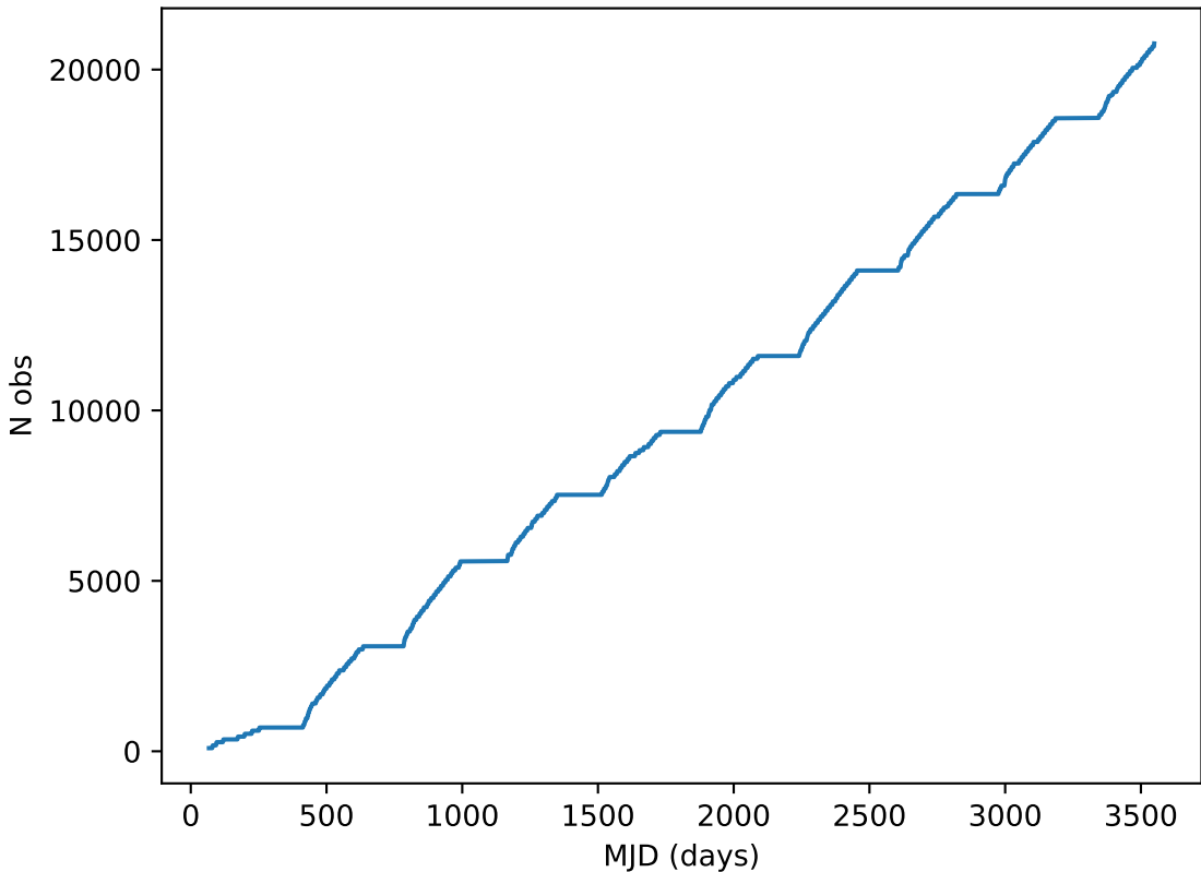
noroll_mjdp0_v3.4_10yrs all bands: DD:ELAISS1 Cumulative NVisits
