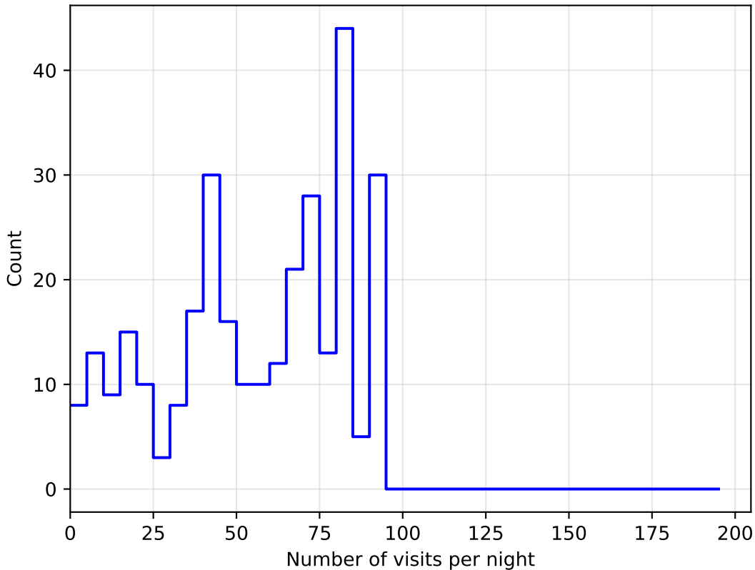
noroll_mjdp0_v3.4_10yrs all bands: DD:EDFS NVisitsPerNight
