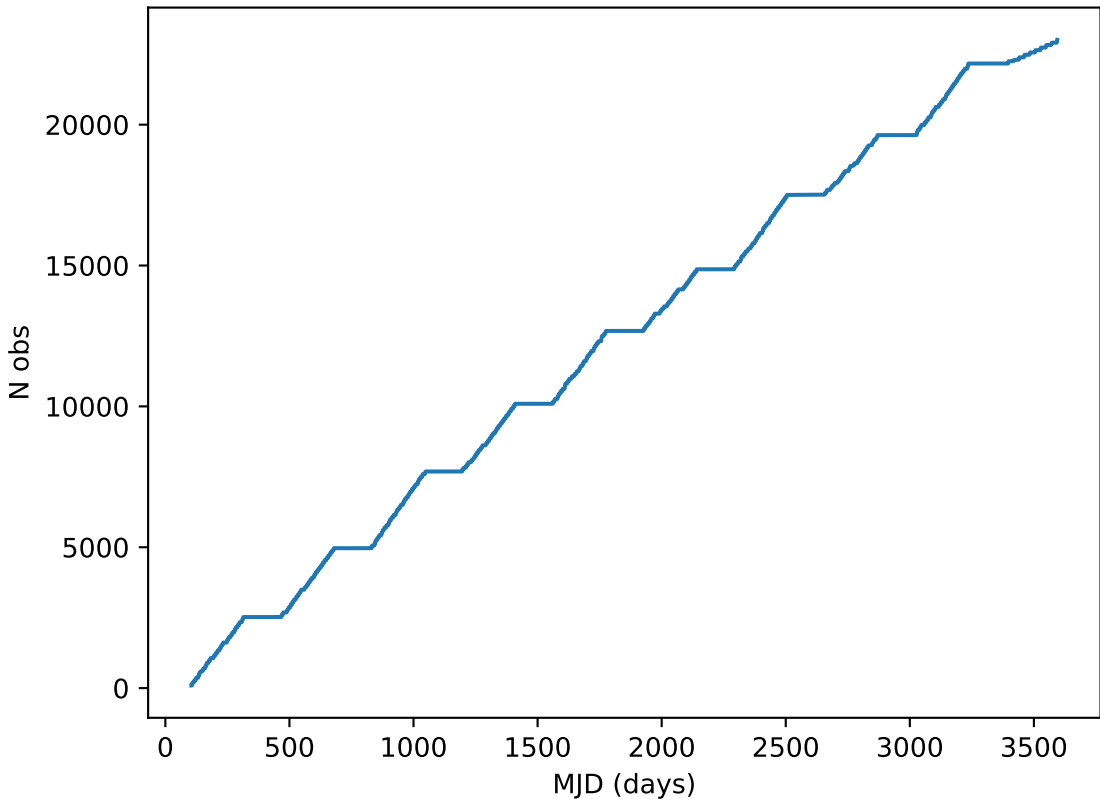
noroll_mjdp0_v3.4_10yrs all bands: DD:EDFS Cumulative NVisits
