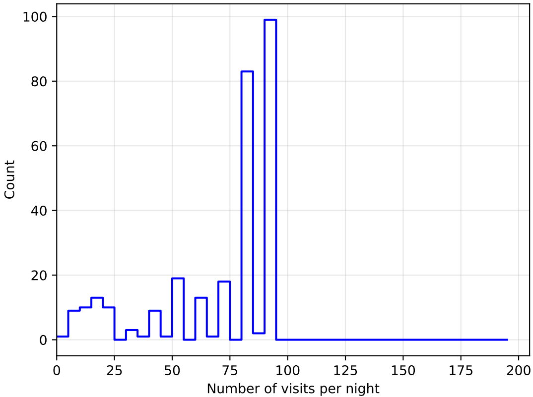
noroll_mjdp0_v3.4_10yrs all bands: DD:ECDFS NVisitsPerNight
