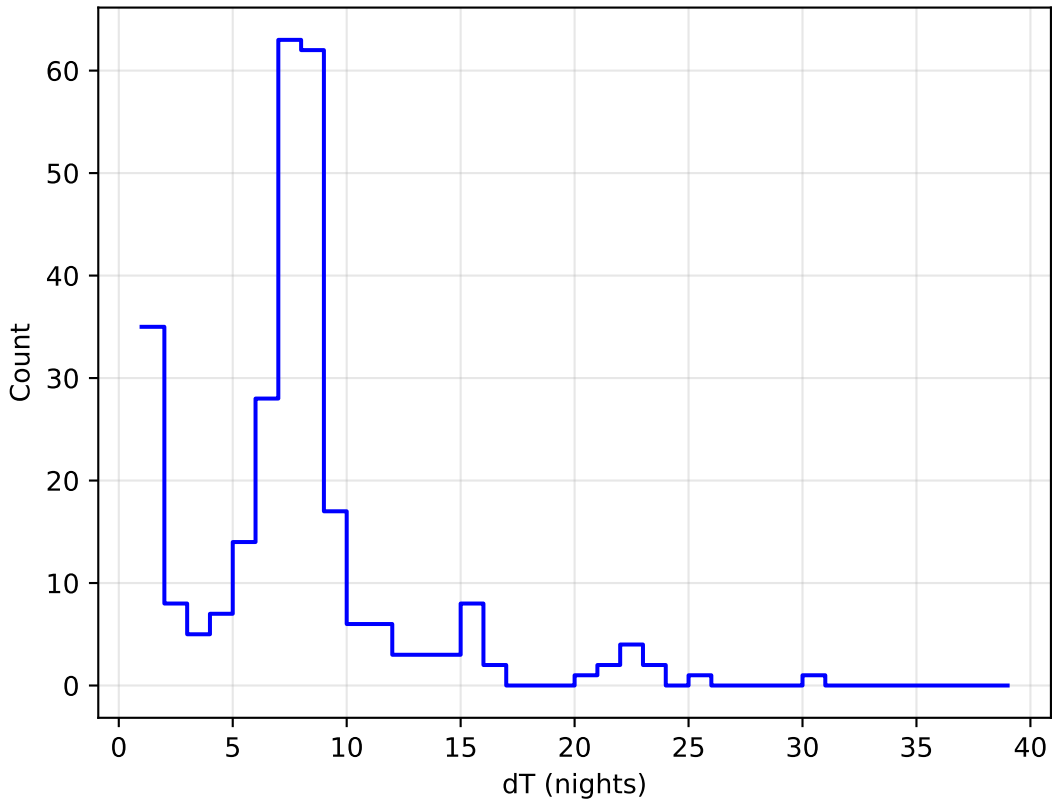
noroll_mjdp0_v3.4_10yrs all bands: DD:ECDFS Delta Nights Histogram
