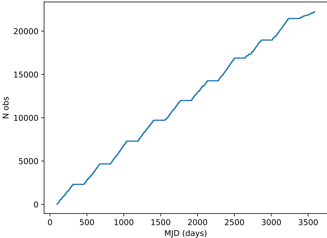
noroll_mjdp0_v3.4_10yrs all bands: DD:ECDFS Cumulative NVisits
